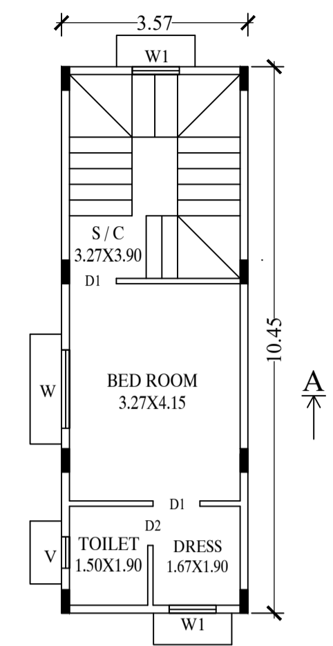
PROPOSED TYPICAL FIRST & SECOND FLOOR PLAN
