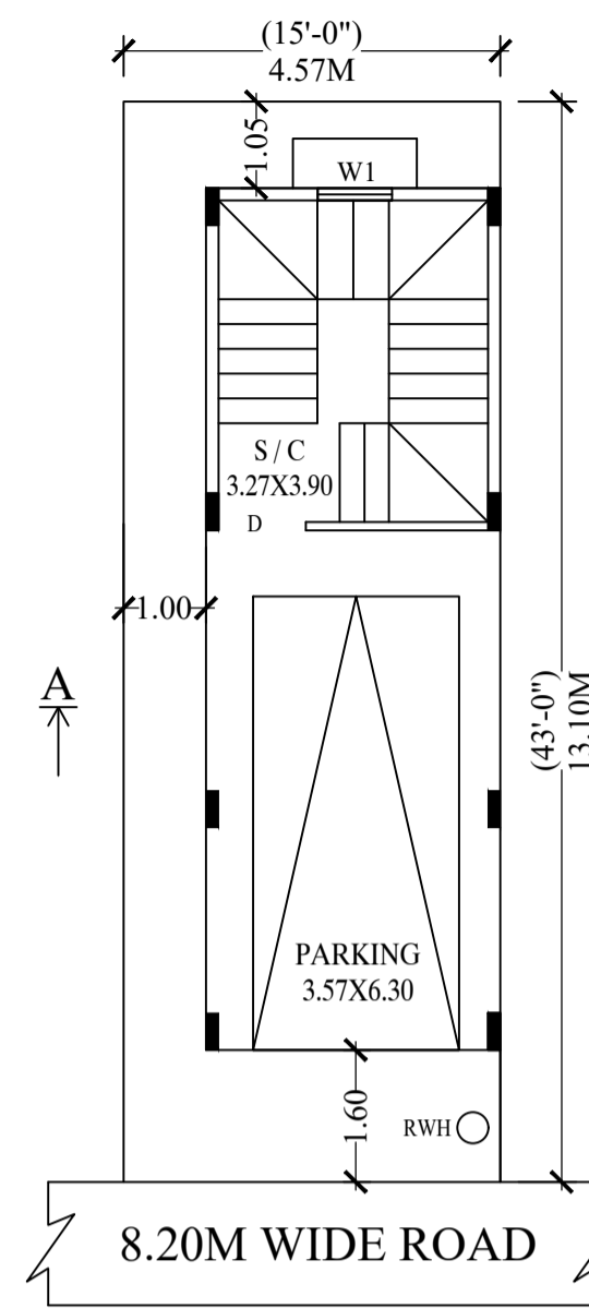
PROPOSED STILT FLOOR PLAN
